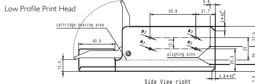
Side View right
