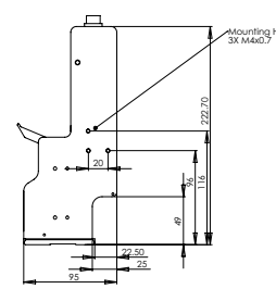
Standard Print Head
